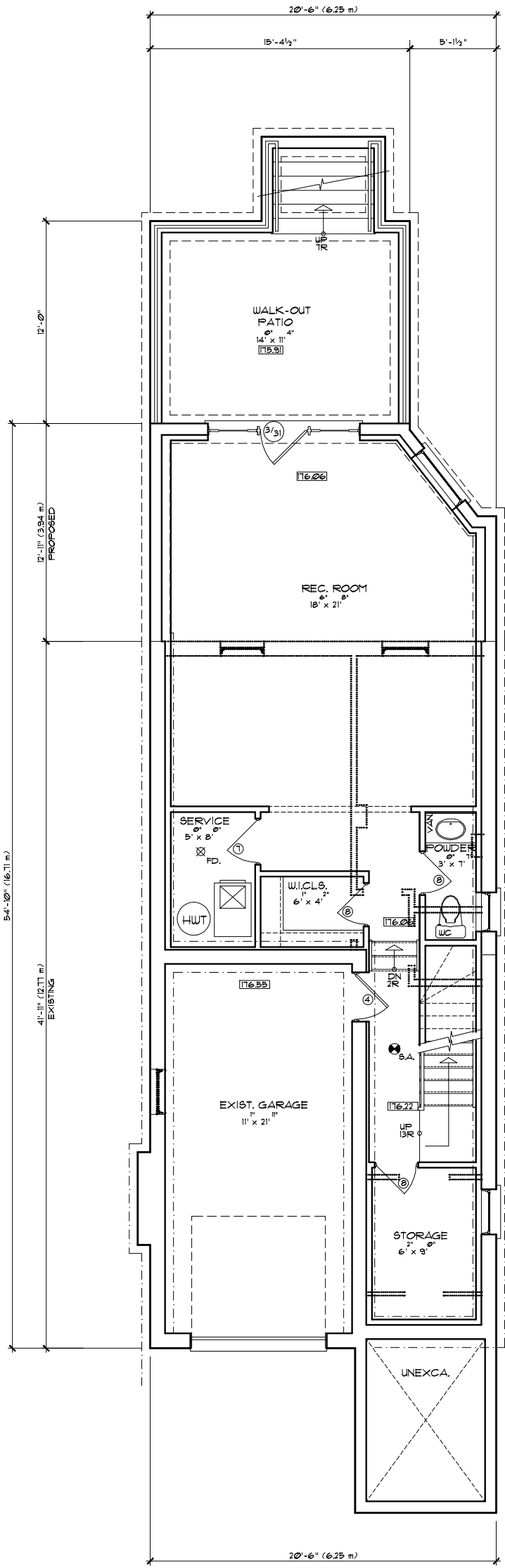
BASEMENT PLAN
