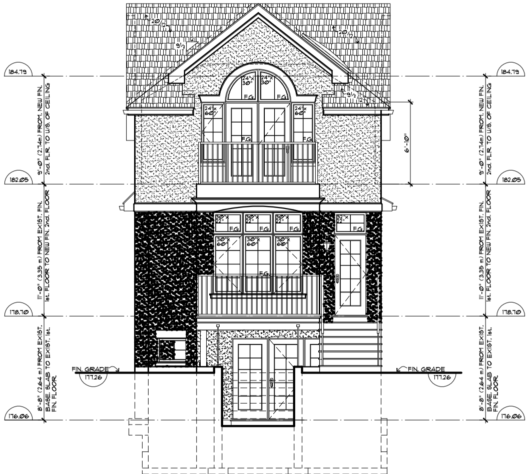
REAR SOUTH ELEVATION
