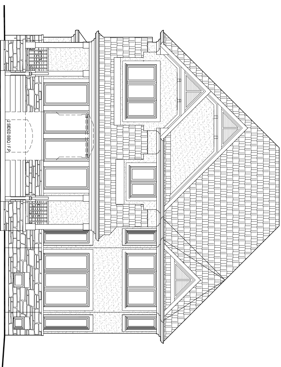
REAR ELEVATION
